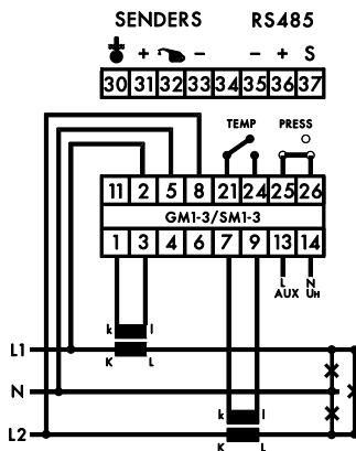
1 Phase 3 Wire Unbalanced Load Connection
