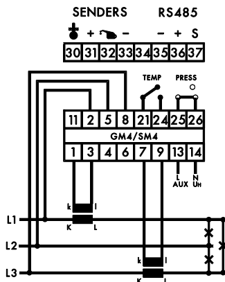
3 Phase 3 Wire Unbalanced Load Connection
