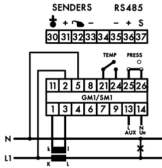
1 Phase Connection
