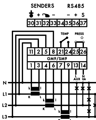
3 Phase 4 Wire Unbalanced Load Connection
